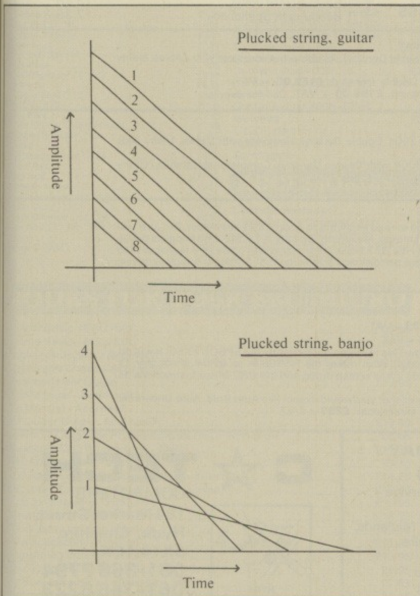
Figure IV: Plucked string, guitar and banjo envelopes
