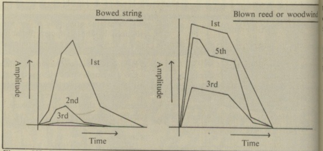
Figure III: Bowed string harmonic envelopes
